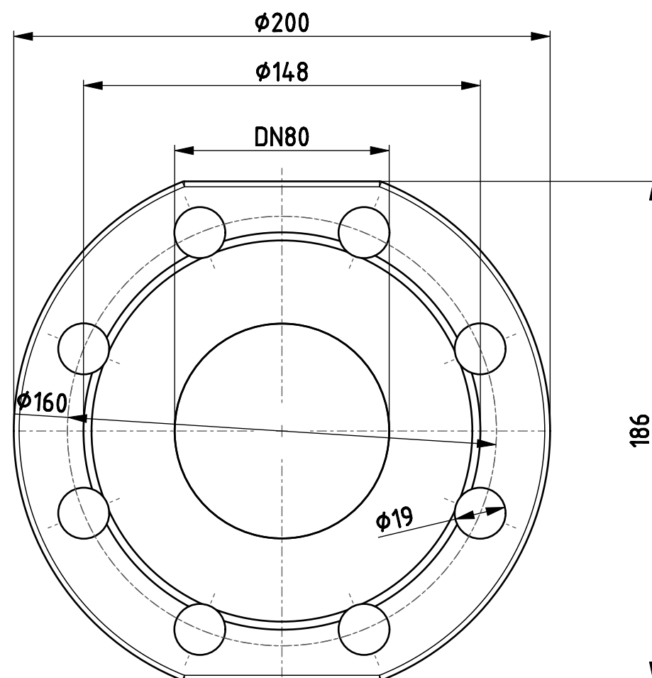
NMTD MAX 80/80-F360 - PN10
