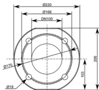
NMTD MAX 100/120-F450- PN6
